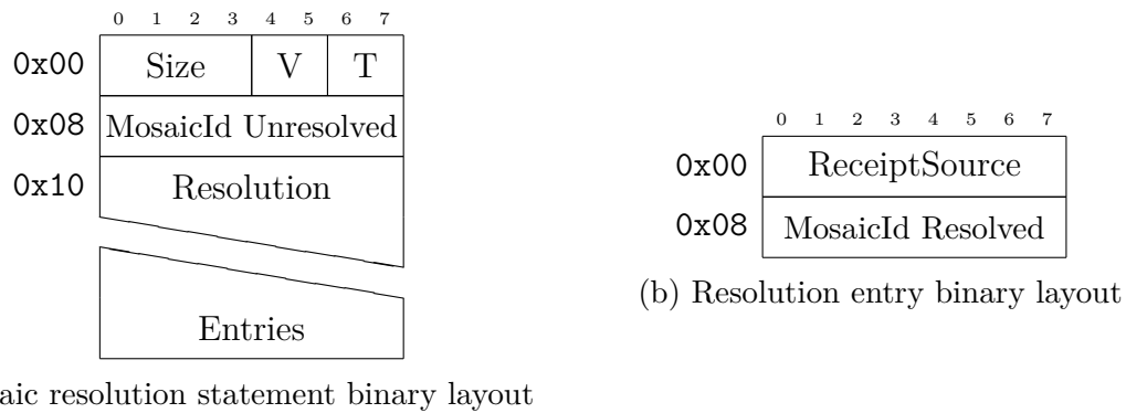
Figure 15: Mosaic resolution statement layout
