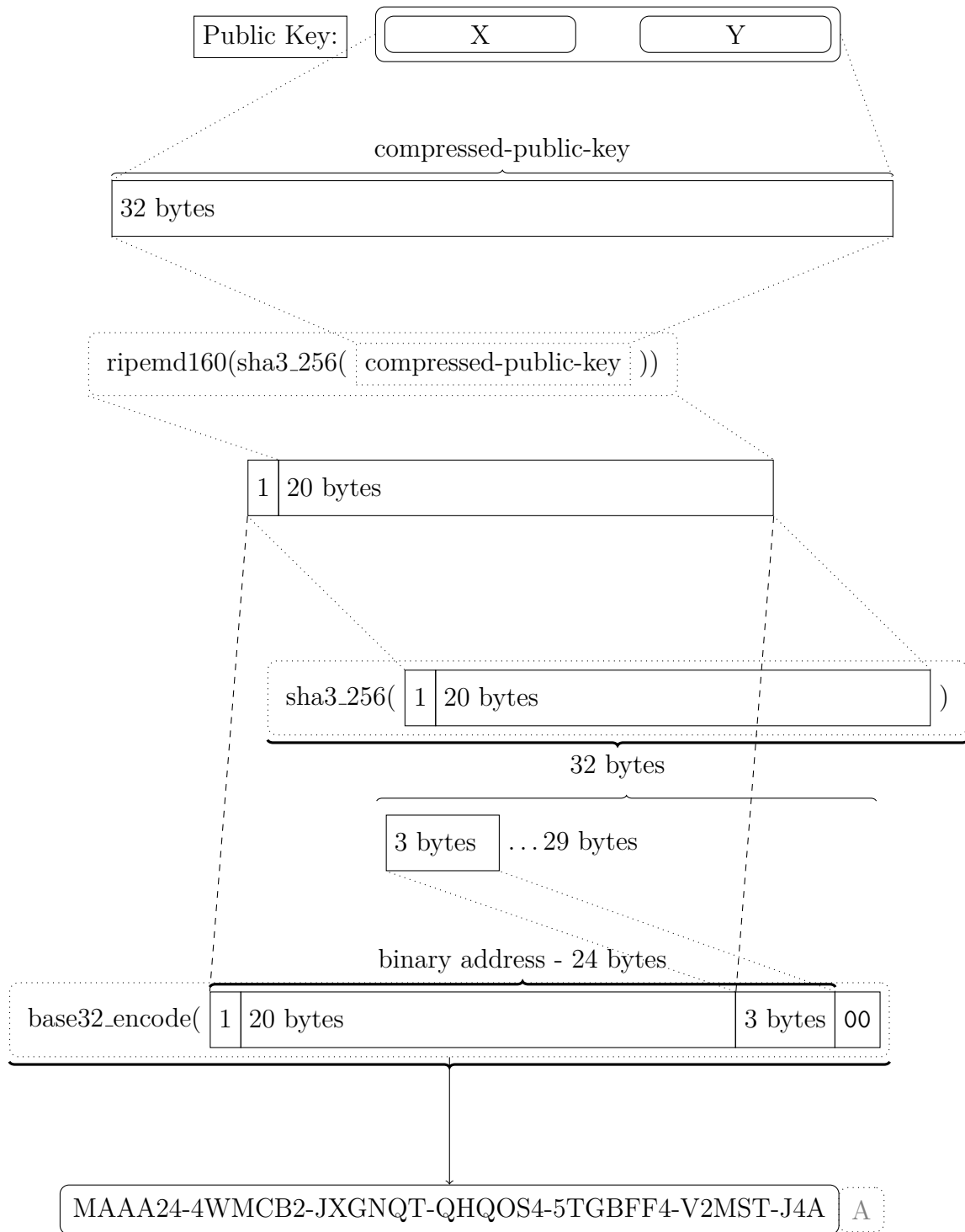
Figure 7: Address generation
