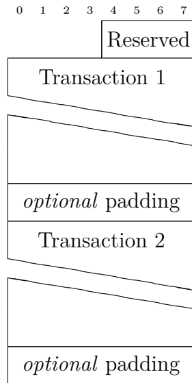
Figure 16: Block transaction footer with padding
