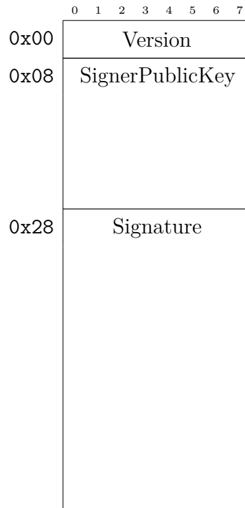
Figure 11: Cosignature binary layout
